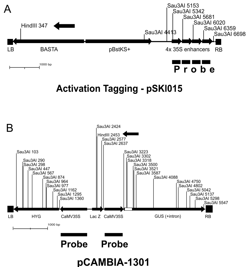
Fig. 1. Schematic representation of the two T-DNA constructs used. Numbers shown with the restriction enzyme sites are the position where the respective enzyme cuts, counting from the left border (LB) towards right border (RB). A: Activation tagging (pSKI015) T-DNA. To facilitate visualization, only the Sau 3AI/ Mbo I sites present in the 35S enhancer region are depicted. The unique Hind III cleavage site is shown and highlighted by a black arrow. The four black square blocks are the regions used as probe, representing sequences of the 35S enhancer. B: pCambia1301 T-DNA. All Sau 3AI/ Mbo I sites are shown. The unique Hind III cleavage site is shown and indicated by a black arrow. White box in the GUS gene represents the catalase intron. Two fat lines are the sequences used as probe (35S sequences).
