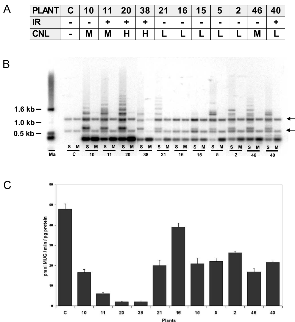
Fig. 3. Analyses of 12 F1 plants generated from the cross of 11 T5 activated tagged plants plus a wild-type plant (Col-0) with a homozygous plant containing a single 35S::GUS insertion. F1 plants obtained from the cross between Col-0 and 35S::GUS are used as control (C). T-DNA copy number levels, methylation status of the 35S enhancer and 35S promoter activity were determined. A: The copy number level (CNL) of the T-DNA activation tagging vector as determined by Southern blot hybridization analyses. The number of T-DNA insertions was determined by measuring the intensity of the hybridizing bands derived from the activation tagging construct (see Fig. 2). The bands derived from the 35S::GUS construct from the pCambia1301 were used as internal control. The plants were categorized in three different 'copy number levels' > five copies). Presence (+) or absence (-) of inverted repeats (IR) determined by PCR using a single primer designed 59 bp upstream of the 4×35S enhancers are indicated. B: Methylation analysis of the F1 plants derived from a cross between activation tagged plants and a homozygous plant with a single copy T-DNA insert containing a 35S::GUS construct (pCambia1301). DNA was digested with Sau3AI (S) and MboI (M), a methylation sensitive and non-sensitive restriction enzyme, respectively. The two bands seen in control (C) represent the pCambia1301 T-DNA insert, and can be used as a loading control. Ma, marker. C: Expression of the GUS transgene in the F1 plants of crosses between 11 different activation tagging T5 plants and Col-0 with a 35S::GUS plant. GUS expression was measured by a MUG assay [13] on four just opened flowers. GUS activity levels were expressed as pmol of methyl-umbelliferone per min per µg of soluble protein (pmol MUG per min per pmol protein). Assays were repeated twice for each plant and the mean values are indicated as bars. The standard deviation of the mean is shown as thin line. C, control plant (F1 of Col-0×35S::GUS).
