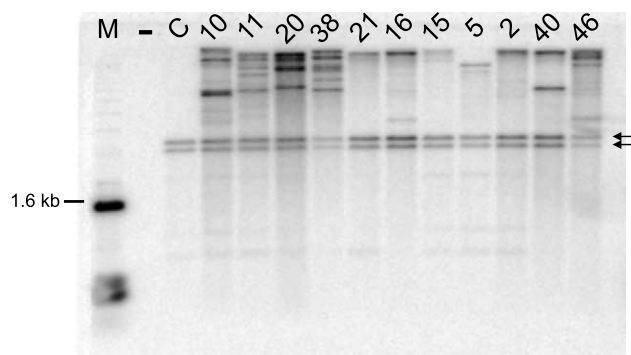
Fig. 2. Southern blot analysis of the 12 F1 plants generated from the cross between 11 selected activation tagging lines (T5) and a plant homozygous for the 35S::GUS construct. Genomic DNA was cut with Hind III and the blot was probed with 35S sequences. The two fragments indicated with arrows are derived from the 35S::GUS construct. C, control plant (F1 of Col-0×35S::GUS). M, marker lane.
